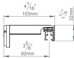
Wall bracket 90 mm
