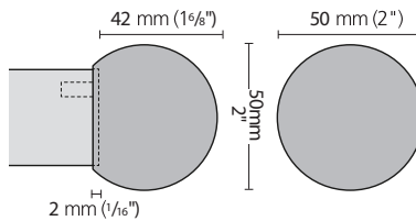
Finial ball 35 mm
