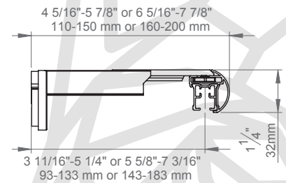
Extendable wall bracket
